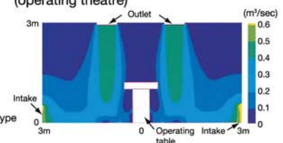
• Air flow distribution diagram (operating theatre)
